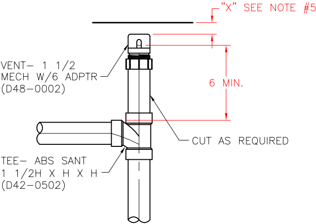
TYPICAL VENT
