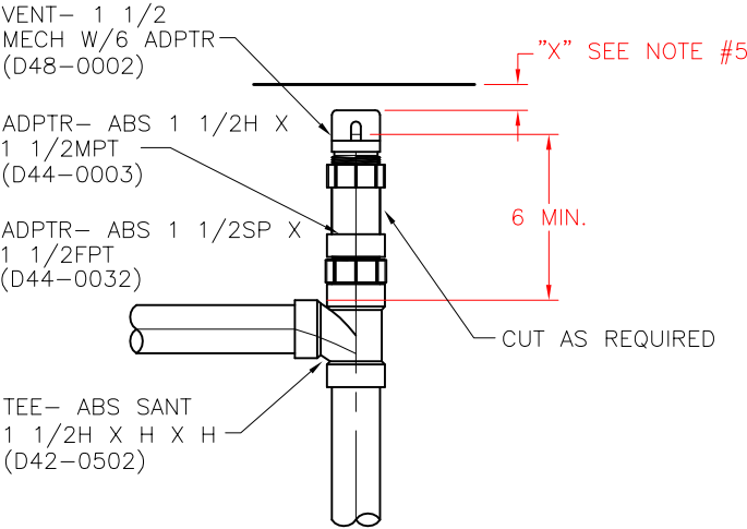
REMOVABLE VENT
